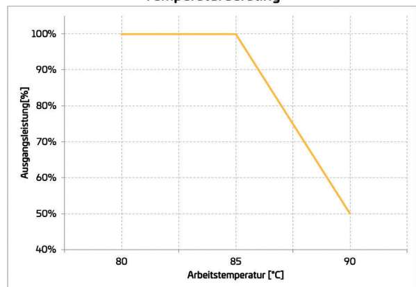
Temperaturderating
